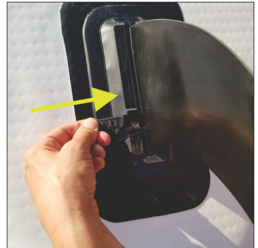
Insert Fin Clips through the holes in the Fins.
