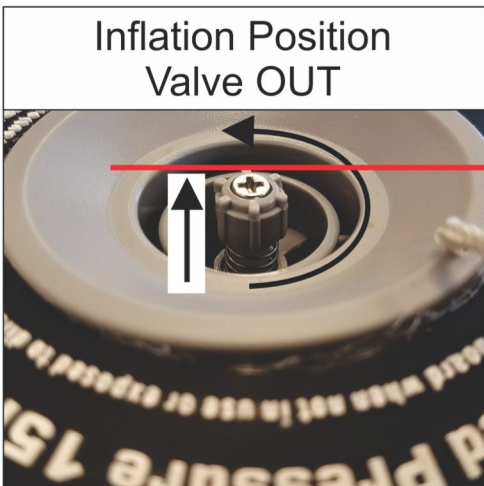
Make sure Valve is in the Outward position by rotating counter clockwise. This allows air to go in but to not escape.
